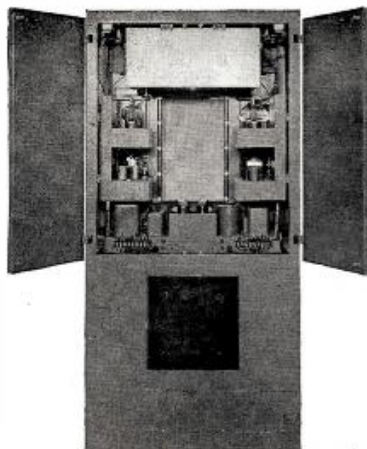
(Left) Collins 300J 250/100 watt AM broadcast transmitter.
